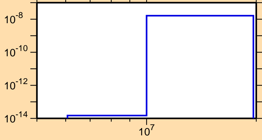
\sigma vs. E for ^{94}\text{Nb}(n,p\alpha)
