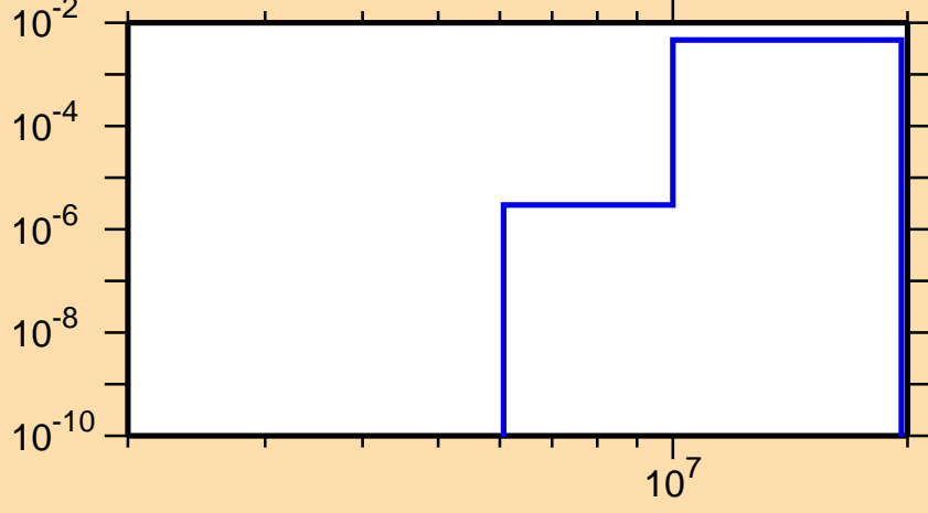
\sigma vs. E for ^{94}\text{Nb}(n,d)
