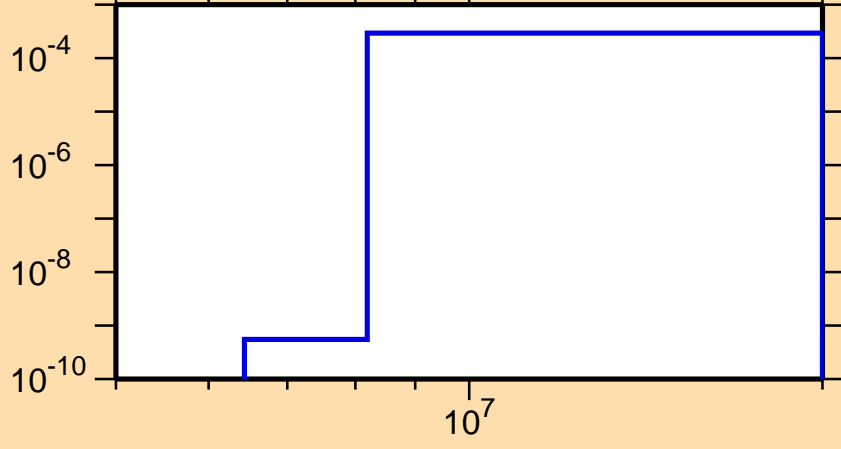
\sigma vs. E for ^{94}\text{Nb}(n,t)
