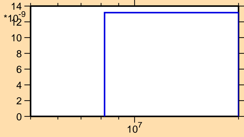
\sigma vs. E for ^{94}\text{Nb}(n,p\alpha)
