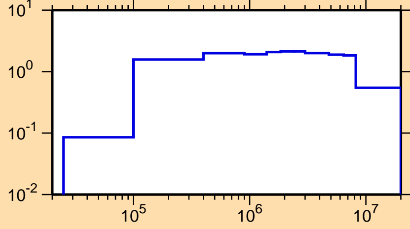
\sigma vs. E for ^{94}\text{Nb}(n,\text{inel.})
