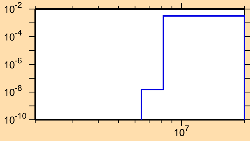
\sigma vs. E for ^{94}\text{Nb}(n,n\alpha)
