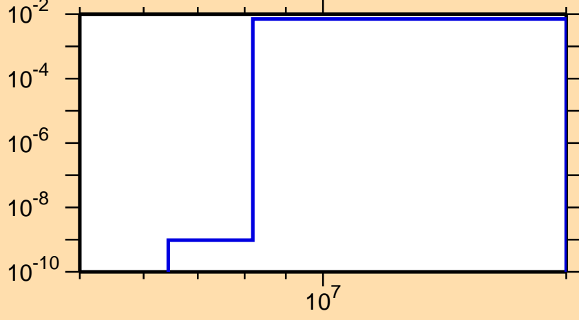
\sigma vs. E for ^{94}\text{Nb}(n,np)
