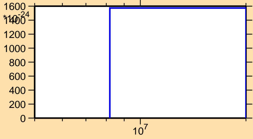
\sigma vs. E for ^{94}\text{Nb}(\text{mt } 11)
