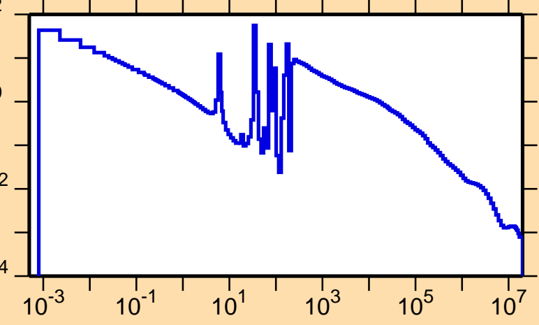
\sigma vs. E for ^{94}\text{Nb}(n,\gamma)
