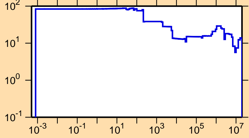
\Delta\sigma/\sigma vs. E for ^{94}\text{Nb}(n,\text{el.})
