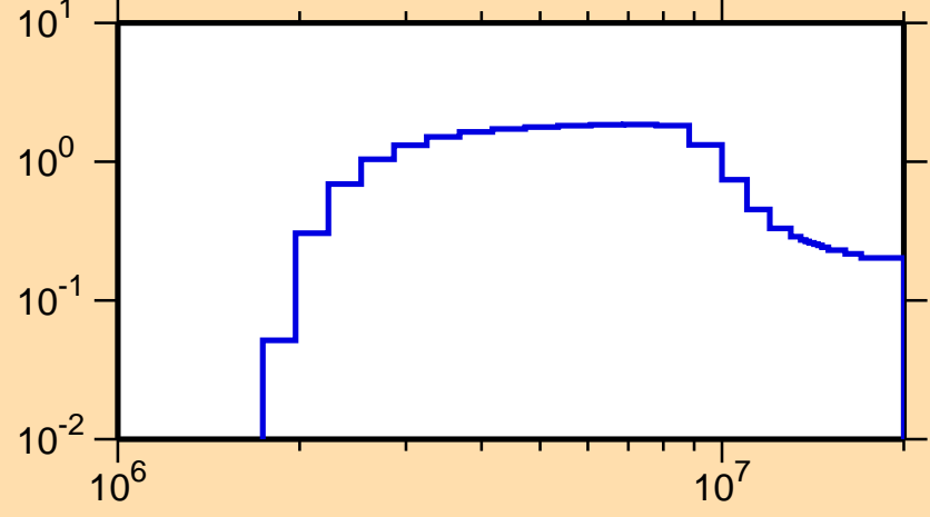
\sigma vs. E for ^{95}\text{Nb}(n,n\text{cont.})
