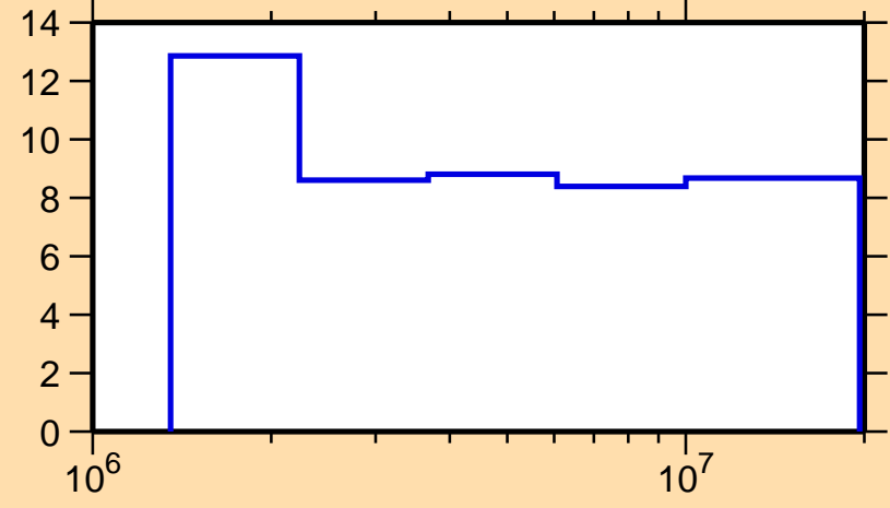
\Delta\sigma/\sigma vs. E for ^{95}\text{Nb}(n,n\text{nonel.})
