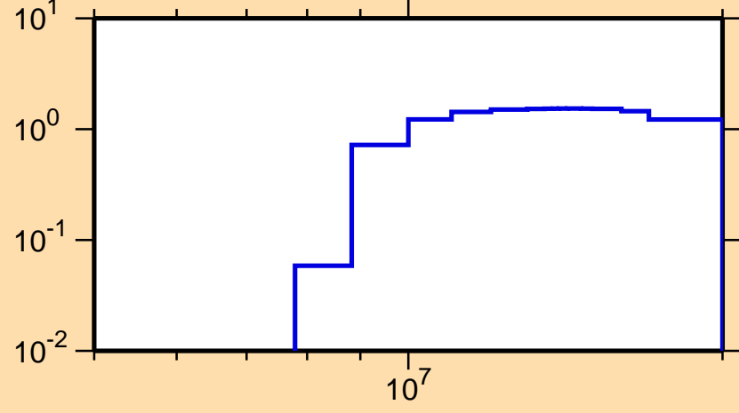
\sigma vs. E for ^{95}\text{Nb}(n,2n)
