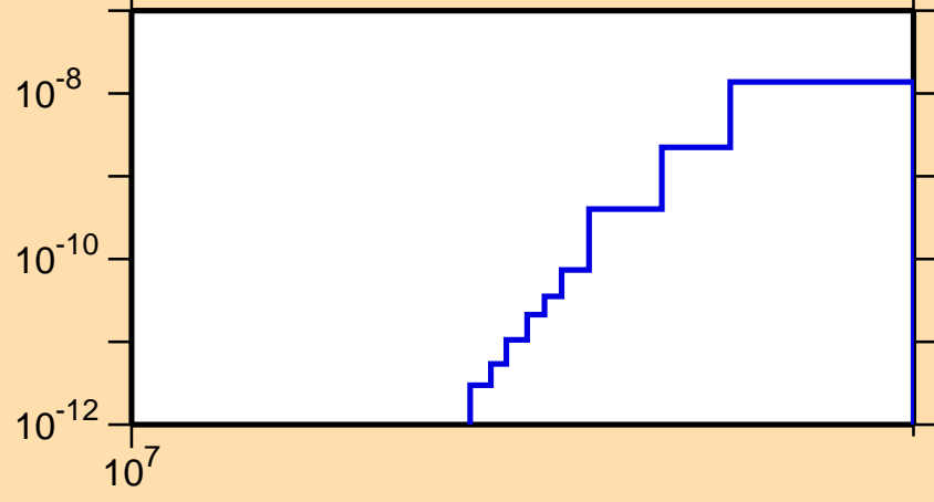
\sigma vs. E for ^{95}\text{Nb}(n,p\alpha)
