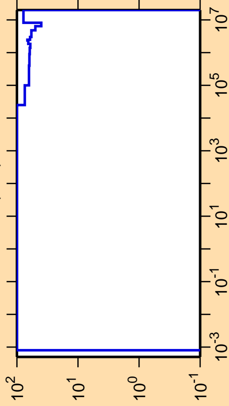
\Delta\sigma/\sigma vs. E for ^{95}\text{Nb}(n,\alpha)
