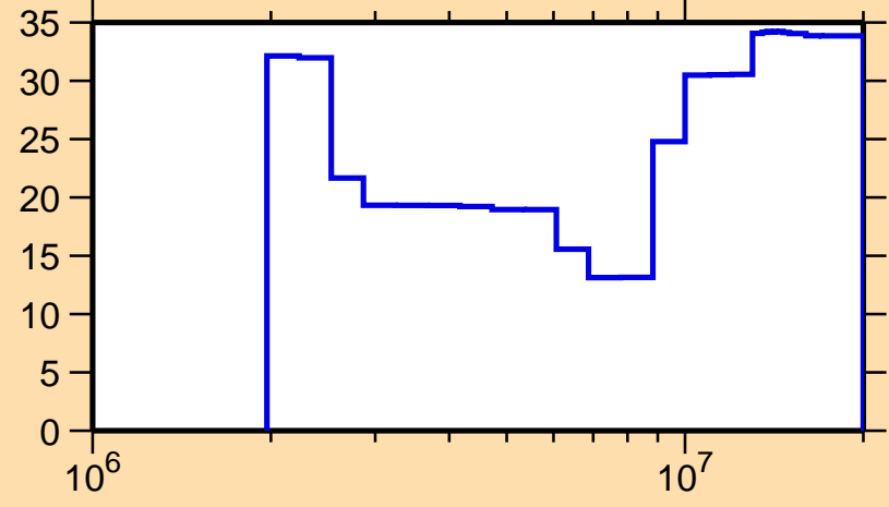
\Delta\sigma/\sigma vs. E for ^{96}\text{Nb}(n,ncont.)
