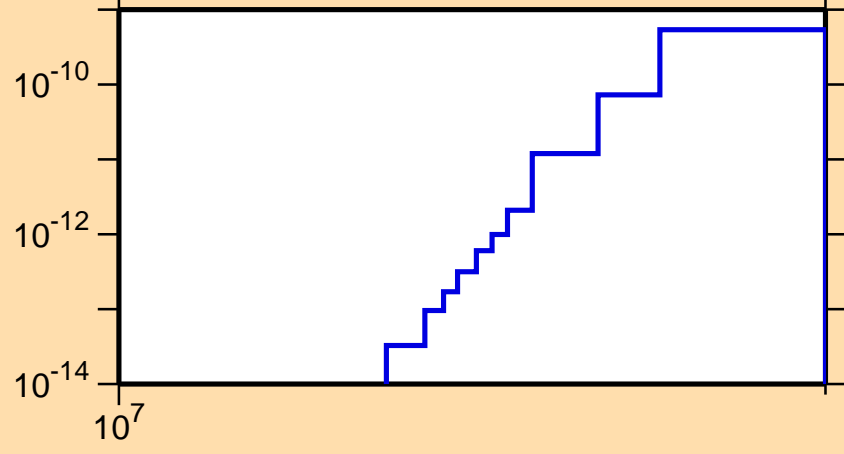
\sigma vs. E for ^{96}\text{Nb}(n,p\alpha)
