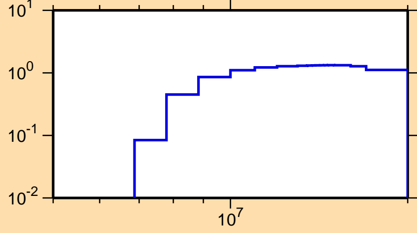
\sigma vs. E for ^{96}\text{Nb}(n,2n)
