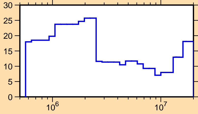
\Delta\sigma/\sigma vs. E for ^{96}\text{Nb}(n,el.)
