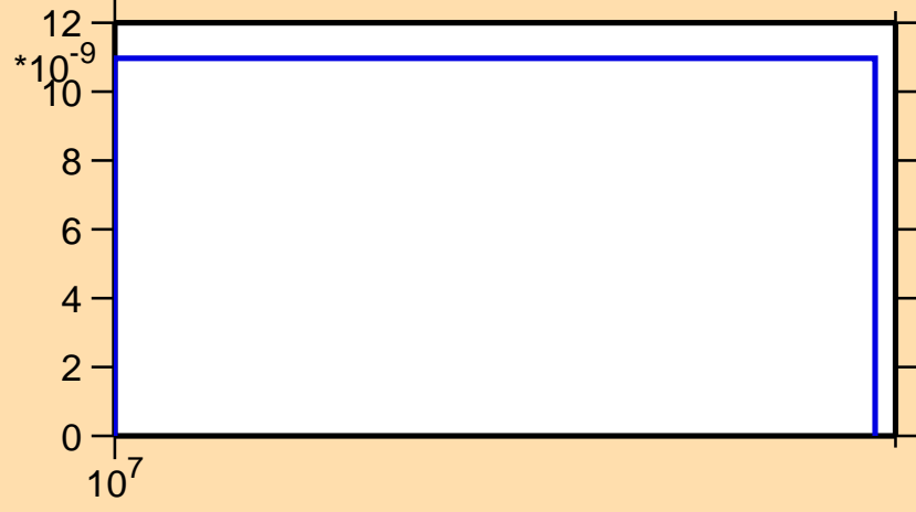
\sigma vs. E for ^{96}\text{Nb}(n,2n\alpha)
