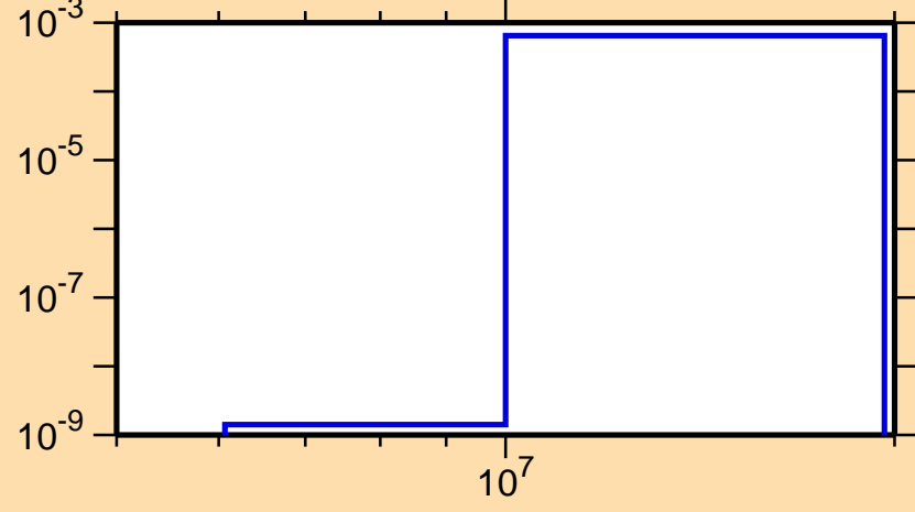
\sigma vs. E for ^{96}\text{Nb}(n,\alpha)
