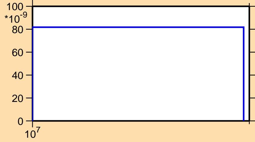
\sigma vs. E for ^{96}\text{Nb}(n,2np)
