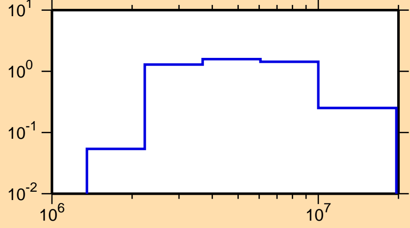
\sigma vs. E for ^{96}\text{Nb}(n,n\text{cont.})
