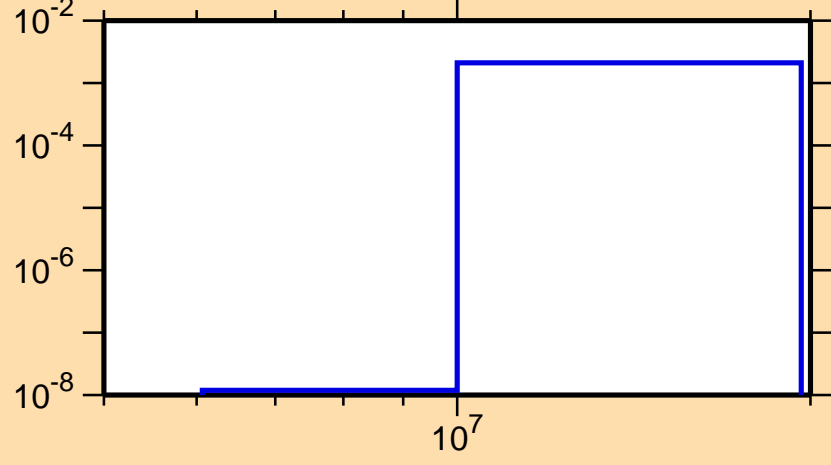
\sigma vs. E for ^{96}\text{Nb}(n,np)
