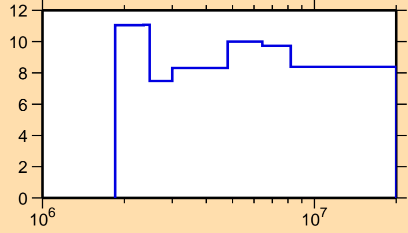
\Delta\sigma/\sigma vs. E for ^{96}\text{Nb}(n,n\text{onel.})
