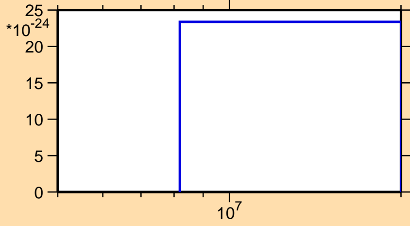
\sigma vs. E for ^{96}\text{Nb}(\text{mt } 11)
