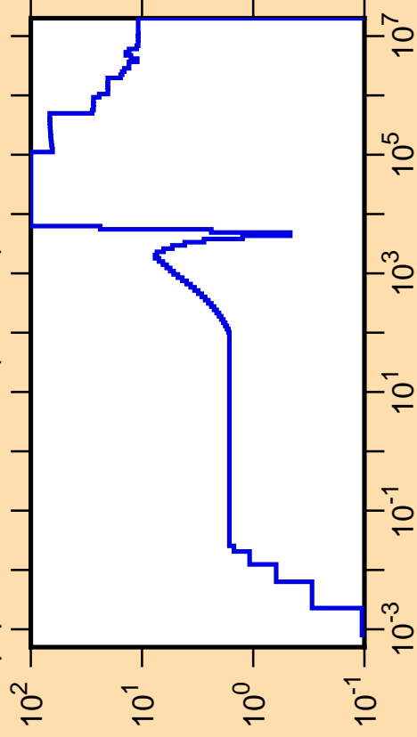
\Delta\mu/\mu vs. E for ^{97}\text{Nb}(\text{mt251})
