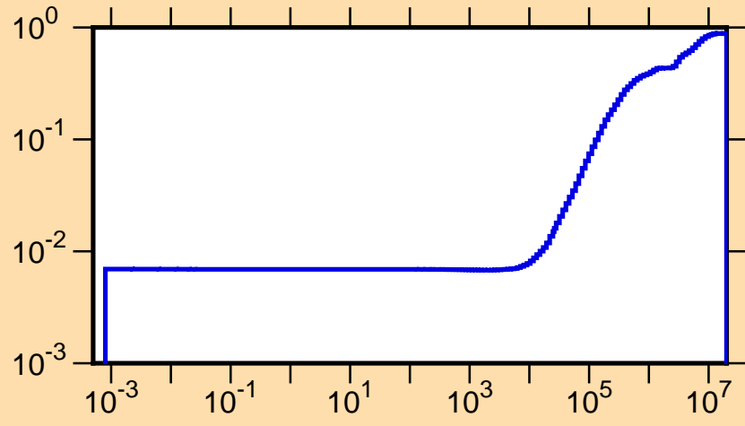
\mu vs. E for ^{97}\text{Nb}(\text{mt251})
