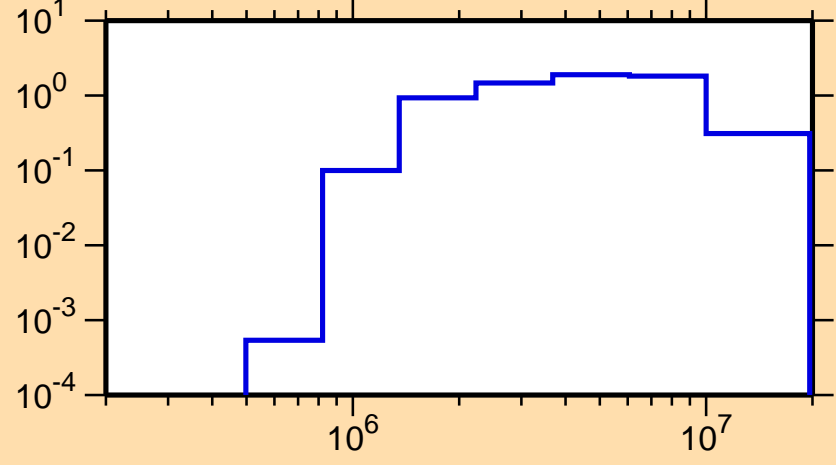
\sigma vs. E for ^{97}\text{Nb}(n,\text{inel.})
