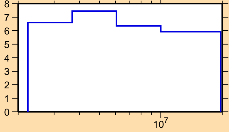
\Delta\sigma/\sigma vs. E for ^{97}\text{Nb}(n,n\text{onel.})
