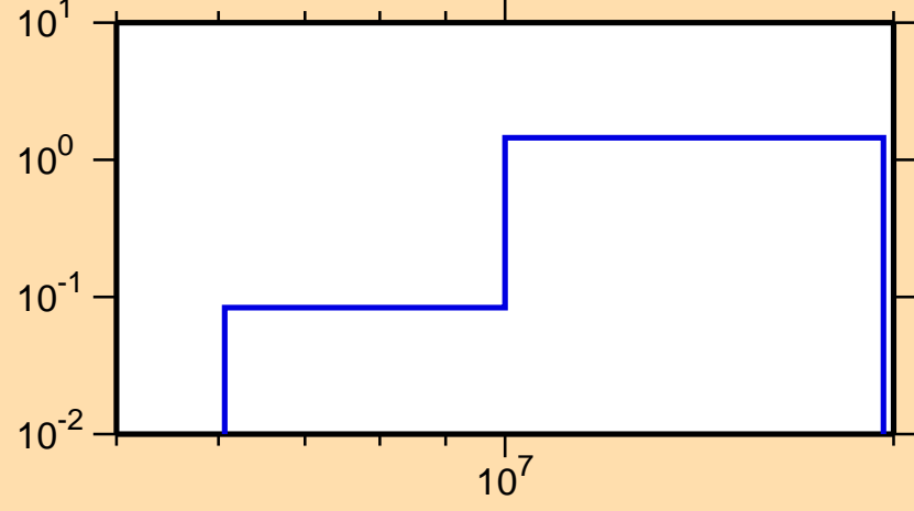
\sigma vs. E for ^{97}\text{Nb}(n,2n)
