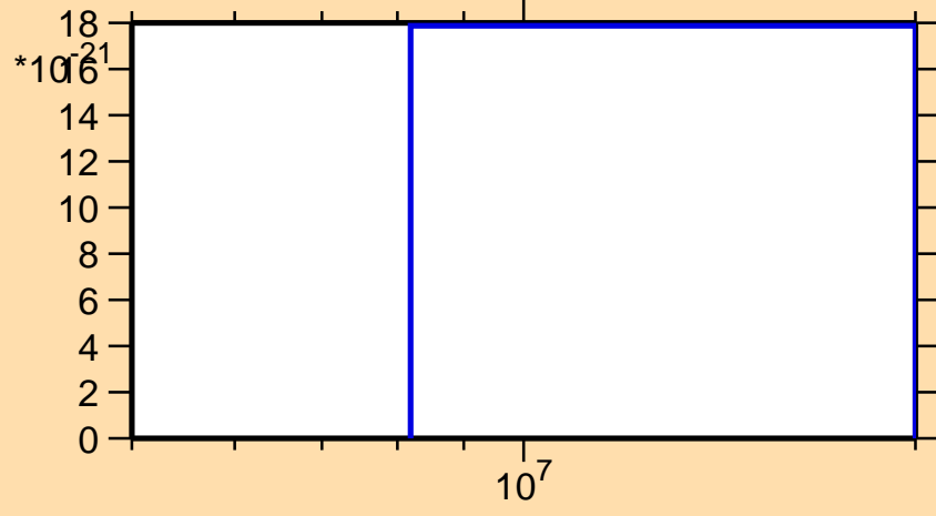
\sigma vs. E for ^{97}\text{Nb}(\text{mt } 34)
