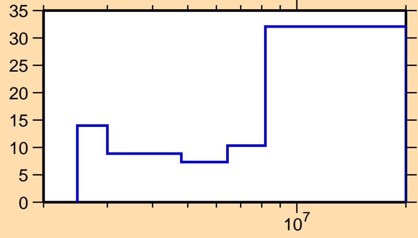
\Delta\sigma/\sigma vs. E for ^{97}\text{Nb}(n,ncont.)
