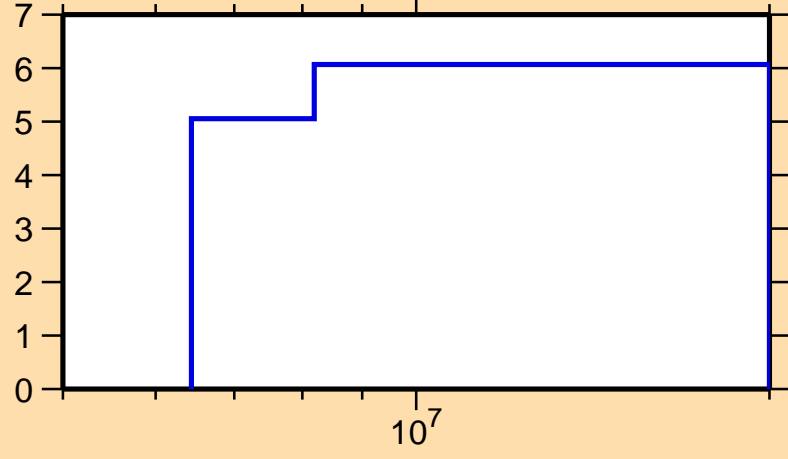
\Delta\sigma/\sigma vs. E for ^{97}\text{Nb}(n,\text{tot.})
