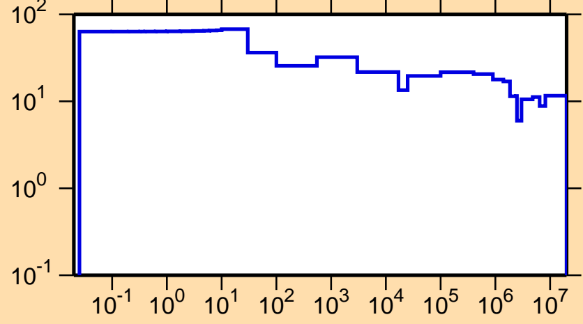
\Delta\sigma/\sigma vs. E for ^{97}\text{Nb}(n,\text{el.})
