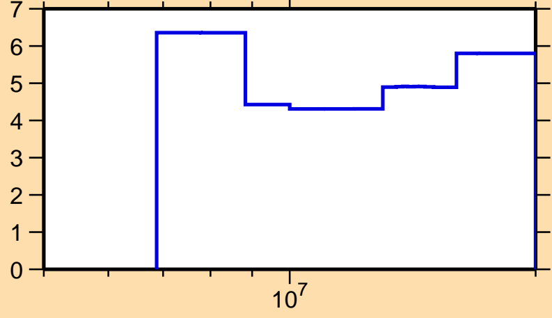
\Delta\sigma/\sigma vs. E for ^{97}\text{Nb}(n,\text{el.})
