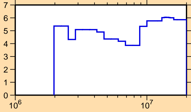
\Delta\sigma/\sigma vs. E for ^{97}\text{Nb}(n,n\text{onrel.})
