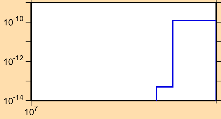
\sigma vs. E for ^{97}\text{Nb}(n,\text{He}3)
