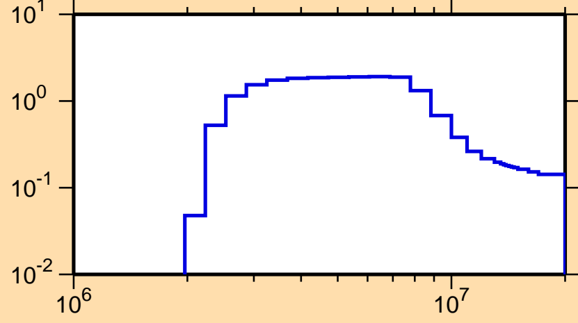
\sigma vs. E for ^{97}\text{Nb}(n,n\text{cont.})
