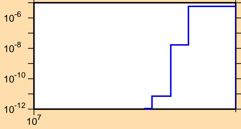
\sigma vs. E for ^{97}\text{Nb}(n,2np)
