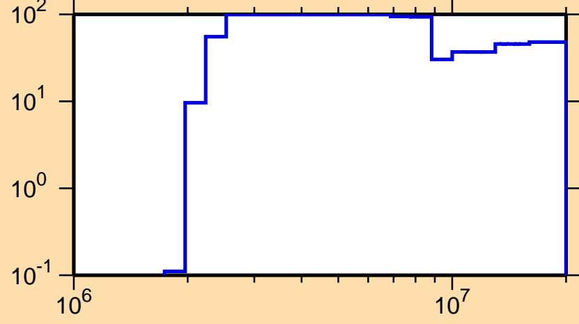
\Delta\sigma/\sigma vs. E for ^{97}\text{Nb}(n,p)
