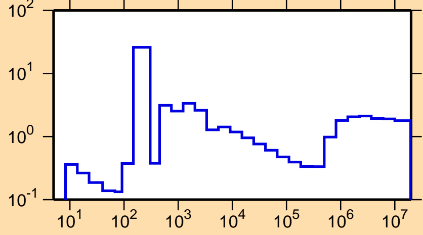
\sigma vs. E for ^{97}\text{Nb}(n,\text{nonel.})
