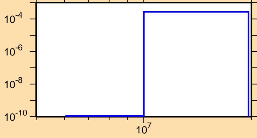
\sigma vs. E for ^{97}\text{Nb}(n,t)
