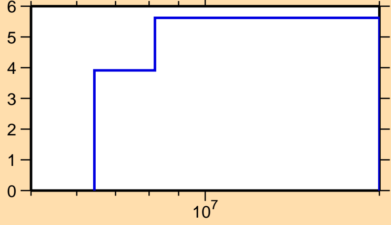
\Delta\sigma/\sigma vs. E for ^{97}\text{Nb}(n,\text{nonel.})
