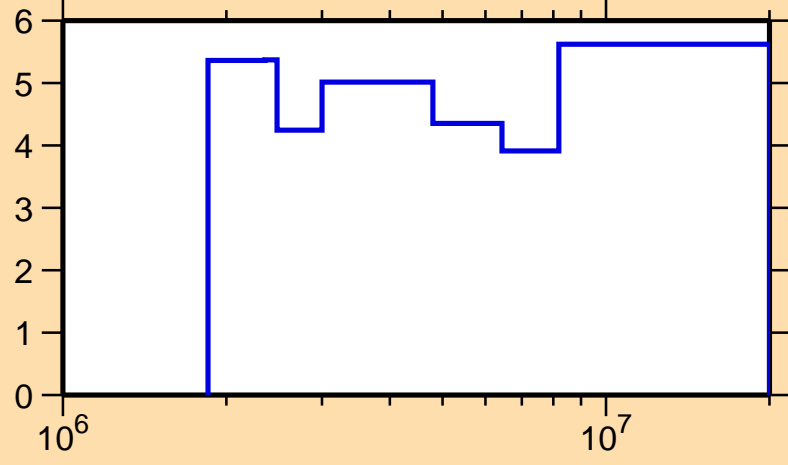
\Delta\sigma/\sigma vs. E for ^{97}\text{Nb}(n,n\text{onel.})
