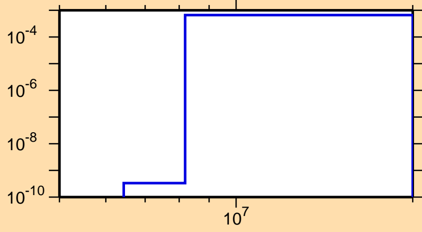
\sigma vs. E for ^{97}\text{Nb}(n,\alpha)
