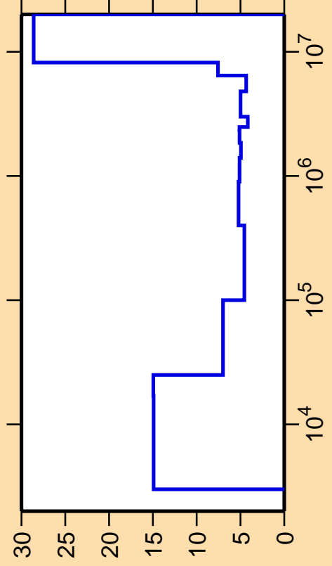
\Delta\sigma/\sigma vs. E for ^{97}\text{Nb}(n,\text{inel.})
