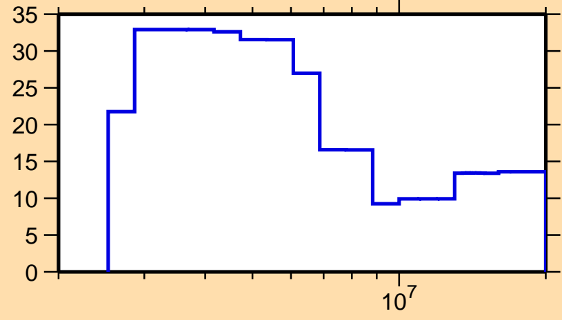
\Delta\sigma/\sigma vs. E for ^{98}\text{Nb}(n,el.)
