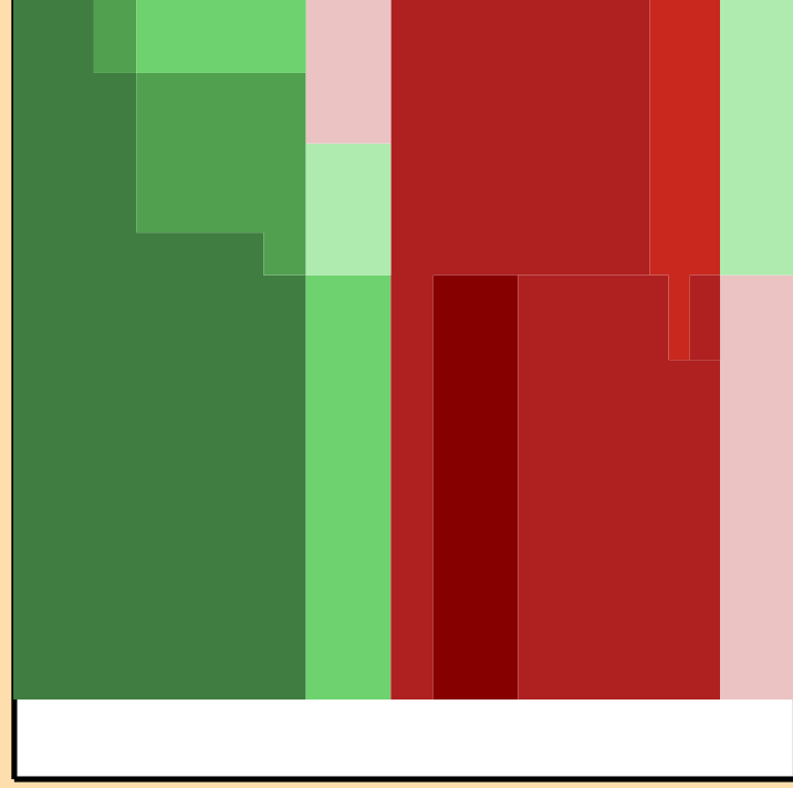
\Delta\sigma/\sigma vs. E for ^{98}\text{Nb}(n,ncont.)
