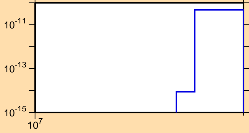
\sigma vs. E for ^{98}\text{Nb}(n,\text{He}3)
