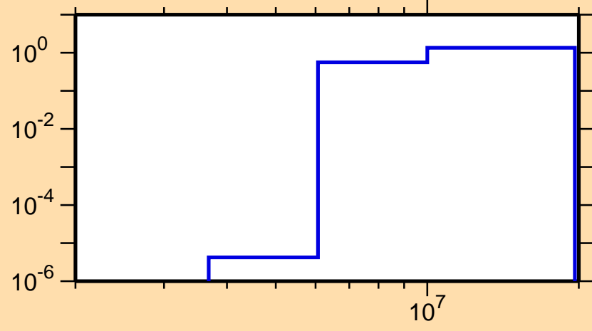
\sigma vs. E for ^{98}\text{Nb}(n,2n)
