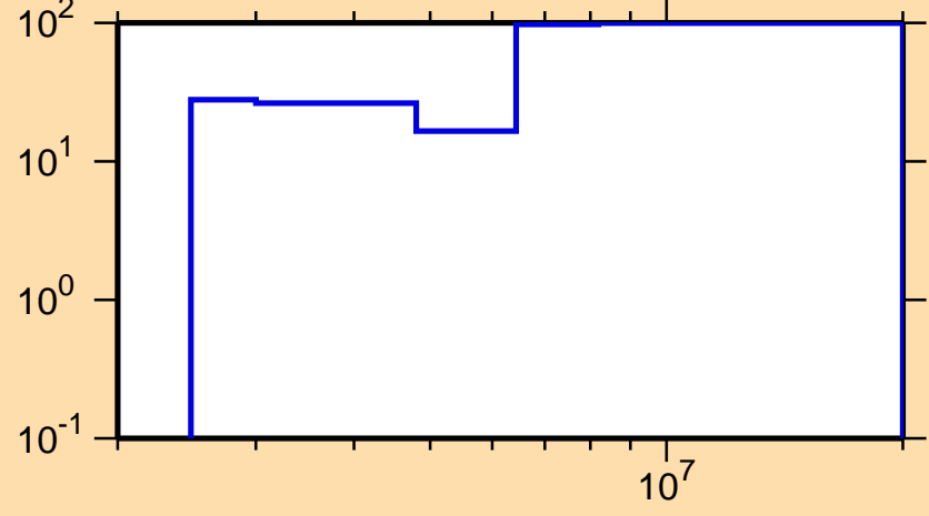
\Delta\sigma/\sigma vs. E for ^{98}\text{Nb}(n,ncont.)
