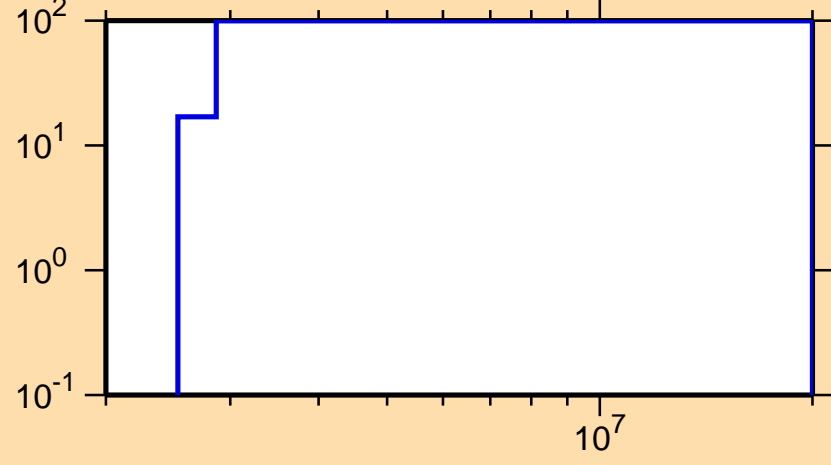
\Delta\sigma/\sigma vs. E for ^{98}\text{Nb}(n,p)
