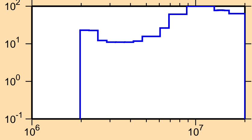
\Delta\sigma/\sigma vs. E for ^{98}\text{Nb}(n,n\text{cont.})
