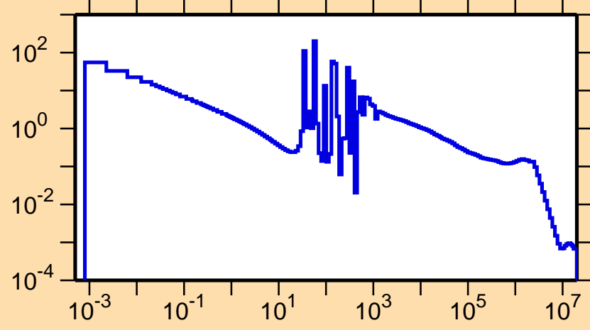
\sigma vs. E for ^{99}\text{Nb}(n,\gamma)
