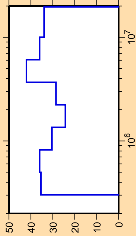
\Delta\sigma/\sigma vs. E for ^{99}\text{Nb}(n,n_1)
