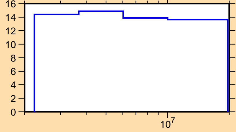
\Delta\sigma/\sigma vs. E for ^{99}\text{Nb}(n,n\text{onel.})
