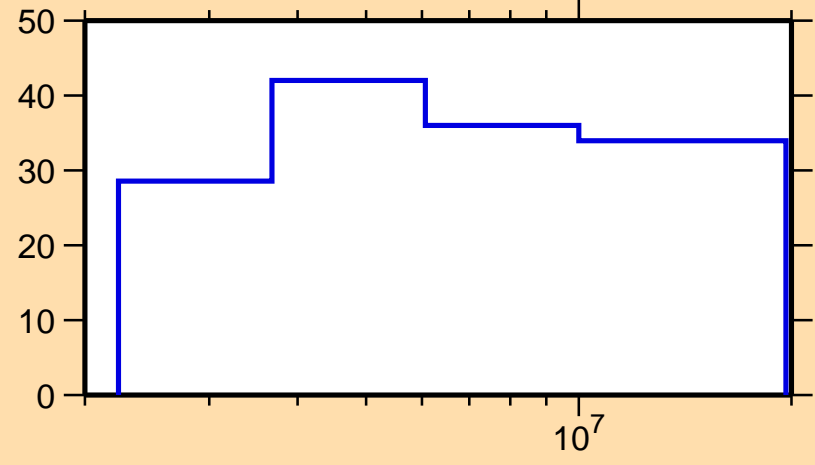
\Delta\sigma/\sigma vs. E for ^{99}\text{Nb}(n, n_1)
