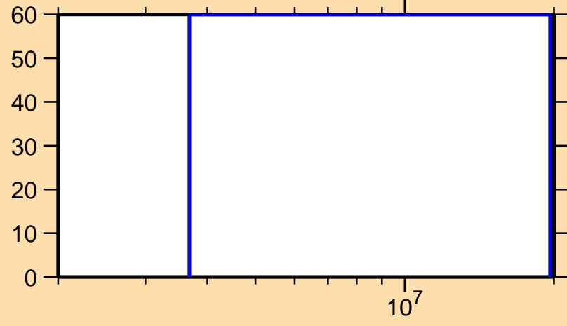
\Delta\sigma/\sigma vs. E for ^{99}\text{Nb}(n,p)
