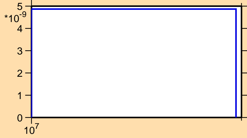
\sigma vs. E for ^{99}\text{Nb}(n,2np)
