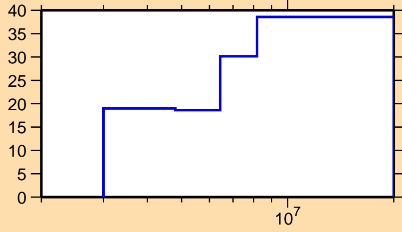
\Delta\sigma/\sigma vs. E for ^{99}\text{Nb}(n,ncont.)
