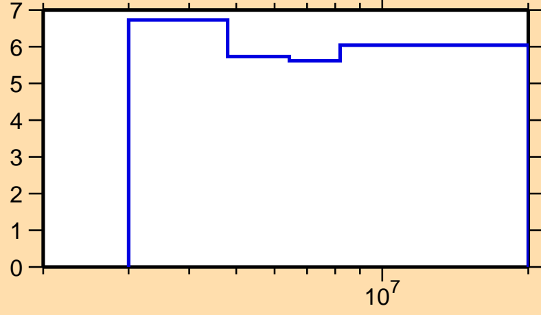
\Delta\sigma/\sigma vs. E for ^{99}\text{Nb}(n,\text{nonel.})
