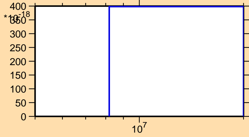
\sigma vs. E for ^{99}\text{Nb}(\text{mt } 11)
