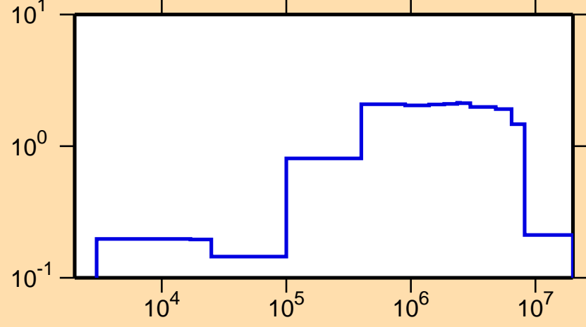
\sigma vs. E for ^{99}\text{Nb}(n,\text{inel.})
