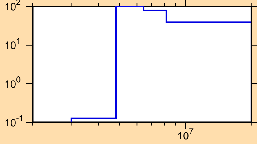
\Delta\sigma/\sigma vs. E for ^{99}\text{Nb}(n,p)
