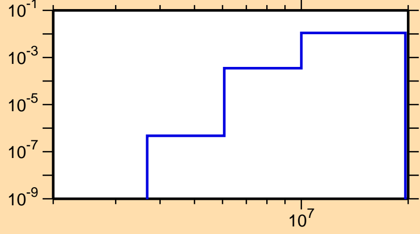
\sigma vs. E for ^{100}\text{Nb}(n,p)
