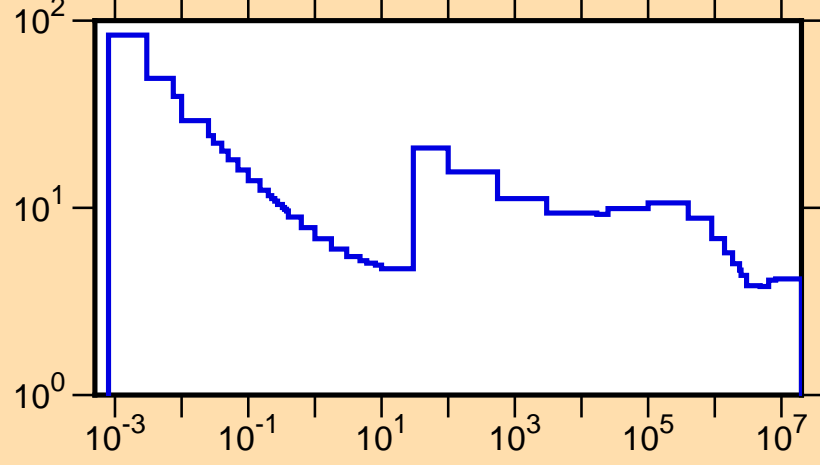
\sigma vs. E for ^{100}\text{Nb}(n,\text{tot.})
