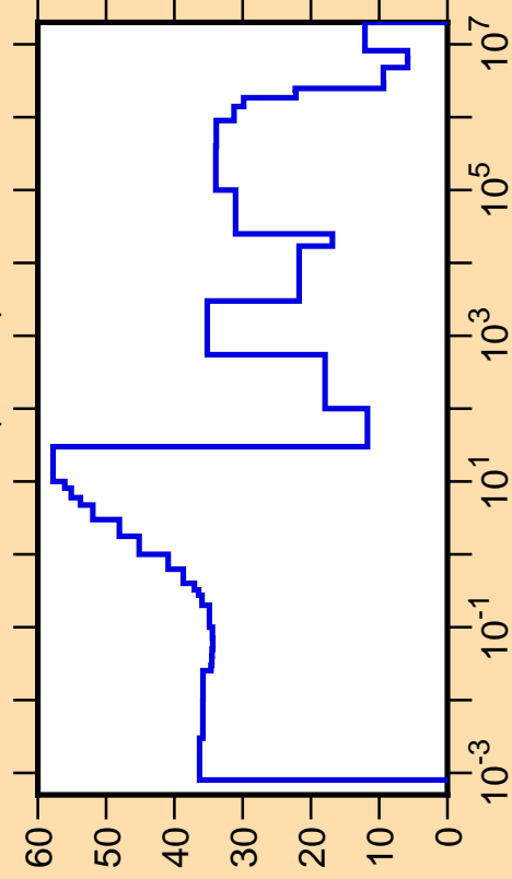
\Delta\sigma/\sigma vs. E for ^{100}\text{Nb}(n,\text{tot.})
