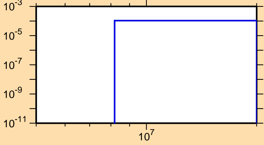
\sigma vs. E for ^{100}\text{Nb}(n,n\alpha)
