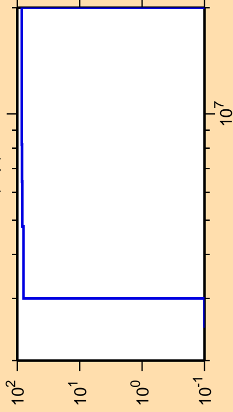
\Delta\sigma/\sigma vs. E for ^{100}\text{Nb}(n,p)
