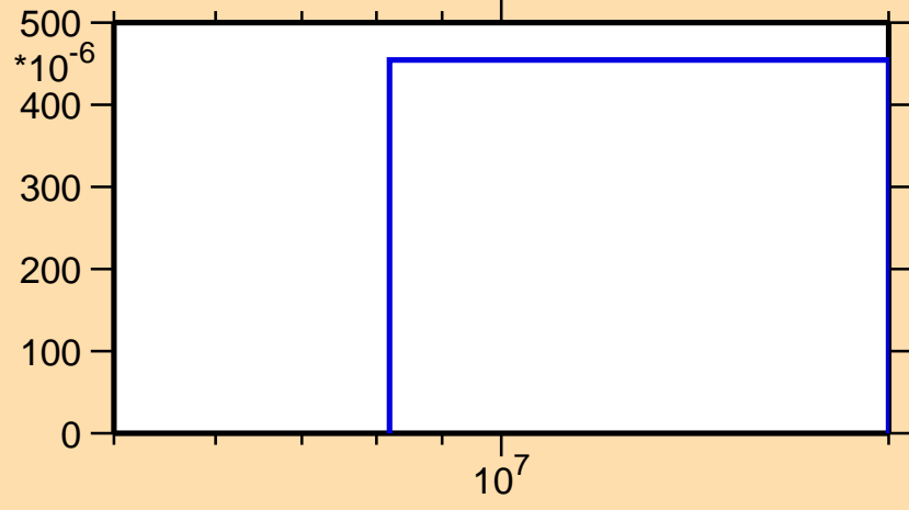
\sigma vs. E for ^{100}\text{Nb}(n,d)
