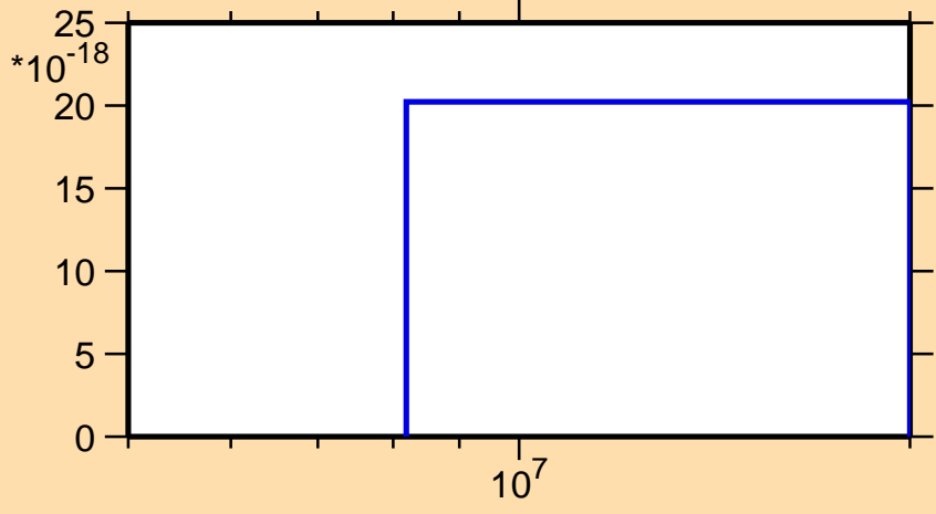
\sigma vs. E for ^{100}\text{Nb}(\text{mt } 11)
