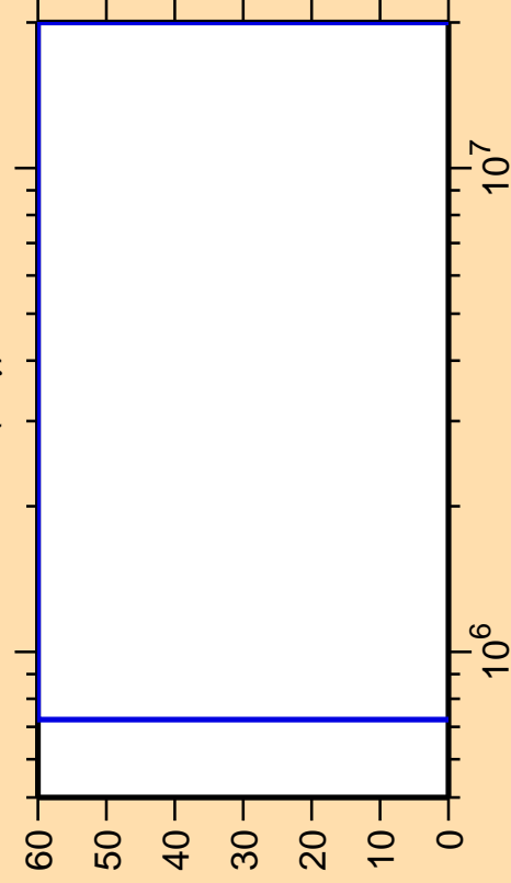
\Delta\sigma/\sigma vs. E for ^{100}\text{Nb}(n,\gamma)
