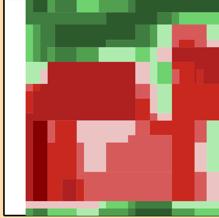
\Delta\sigma/\sigma vs. E for ^{100}\text{Nb}(n,n\text{cont.})
