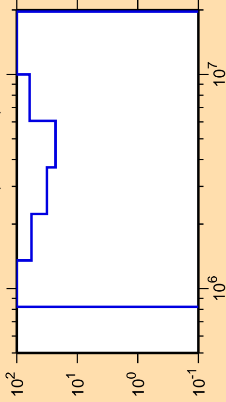
\Delta\sigma/\sigma vs. E for ^{101}\text{Nb}(n,n\text{cont.})
