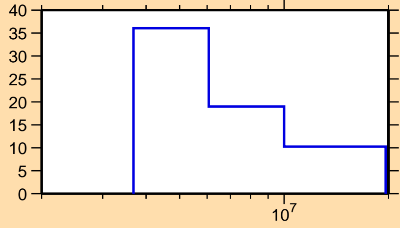
\Delta\sigma/\sigma vs. E for ^{101}\text{Nb}(n,el.)
