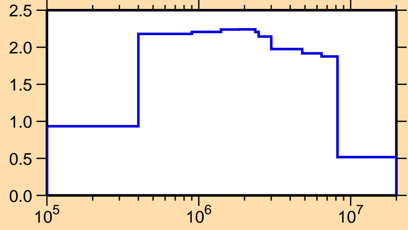
\sigma vs. E for ^{101}\text{Nb}(n,\text{inel.})
