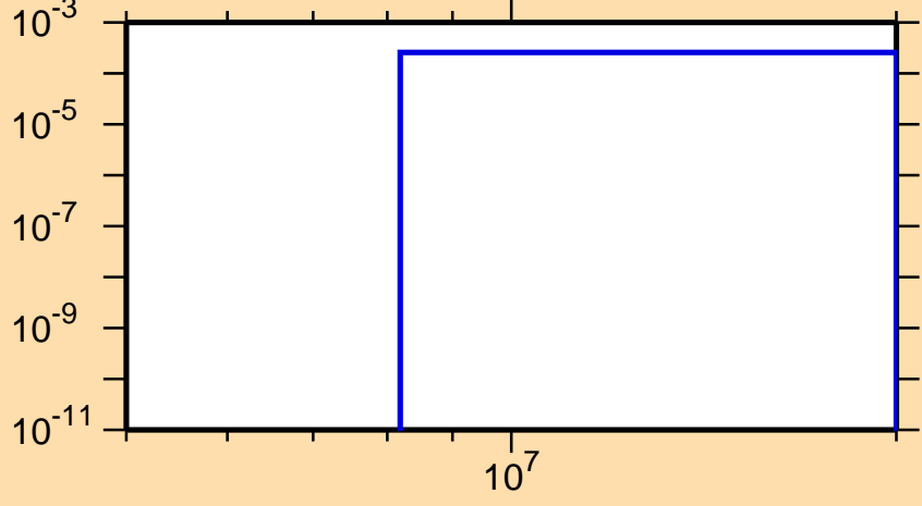
\sigma vs. E for ^{101}\text{Nb}(n,d)
