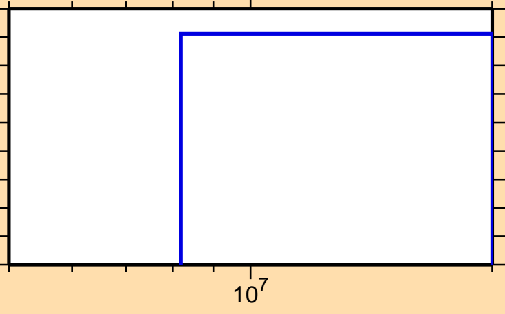
\sigma vs. E for ^{101}\text{Nb}(n,t)
