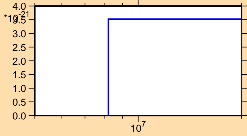
\sigma vs. E for ^{101}\text{Nb}(\text{mt } 11)
