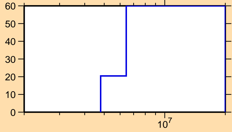
\Delta\sigma/\sigma vs. E for ^{101}\text{Nb}(n,ncont.)
