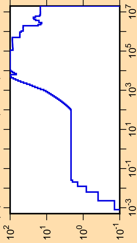
\Delta\mu/\mu vs. E for ^{102}\text{Nb}(\text{mt251})
