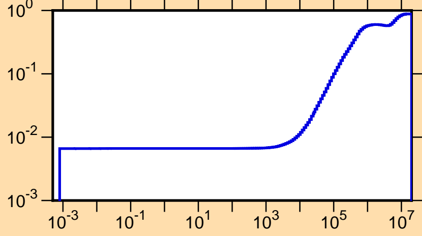
\mu vs. E for ^{102}\text{Nb}(\text{mt251})
