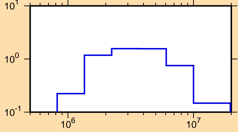
\sigma vs. E for ^{102}\text{Nb}(n,n\text{cont.})
