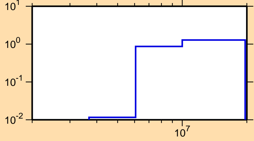
\sigma vs. E for ^{102}\text{Nb}(n,2n)
