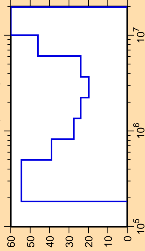
\Delta\sigma/\sigma vs. E for ^{102}\text{Nb}(n,\text{inel.})
