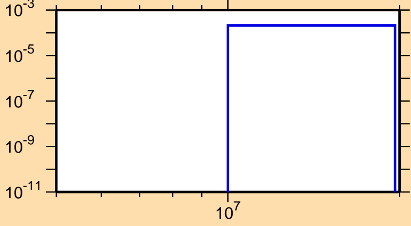
\sigma vs. E for ^{102}\text{Nb}(n,d)
