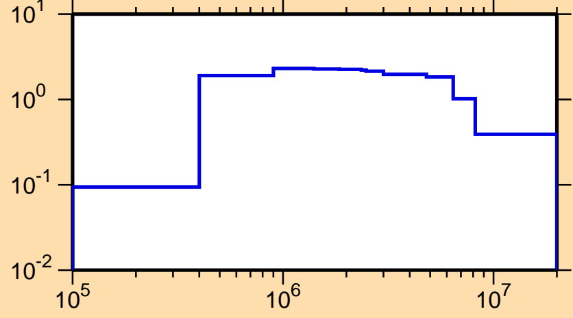
\sigma vs. E for ^{102}\text{Nb}(n,\text{inel.})
