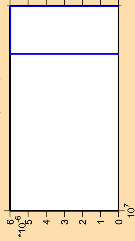
\Delta\sigma/\sigma vs. E for ^{104}\text{Nb}(n,3n\alpha)
