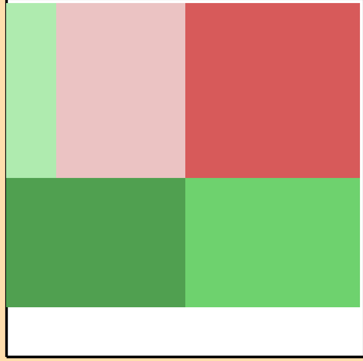
\Delta\sigma/\sigma vs. E for ^{104}\text{Nb}(n,\gamma)
