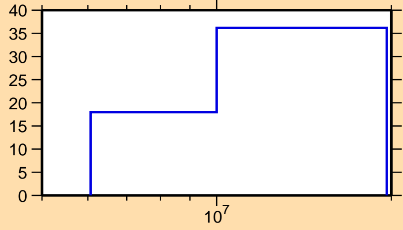
\Delta\sigma/\sigma vs. E for ^{104}\text{Nb}(n,el.)
