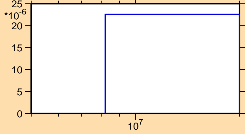
\sigma vs. E for ^{104}\text{Nb}(n,t)
