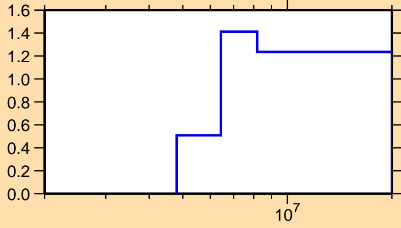
\sigma vs. E for ^{104}\text{Nb}(n,2n)
