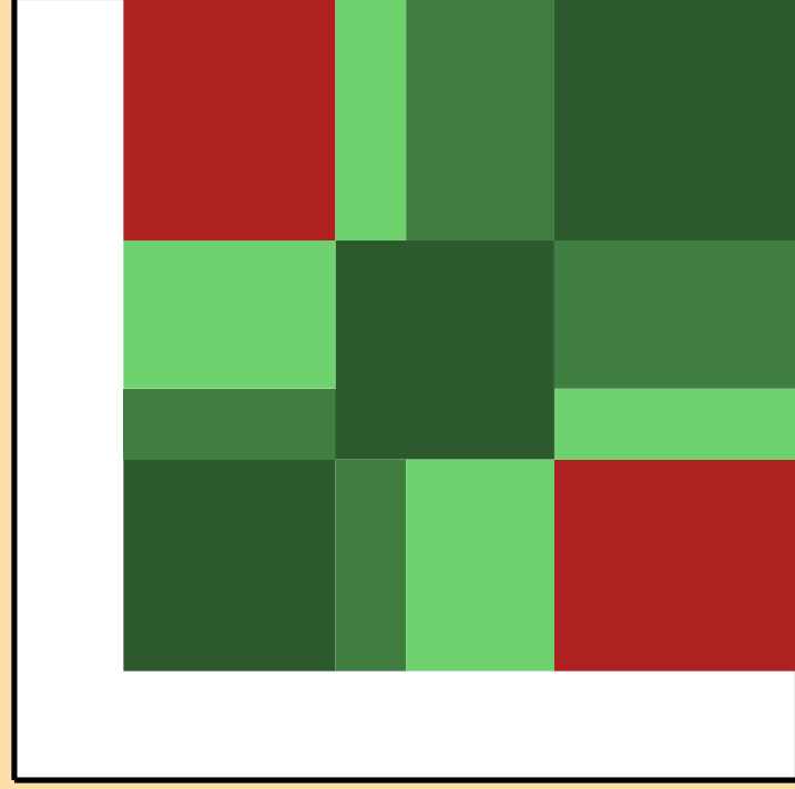
\sigma vs. E for ^{105}\text{Nb}(n,2n)
