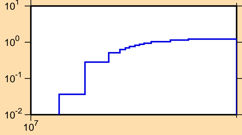
\sigma vs. E for ^{105}\text{Nb}(n,3n)
