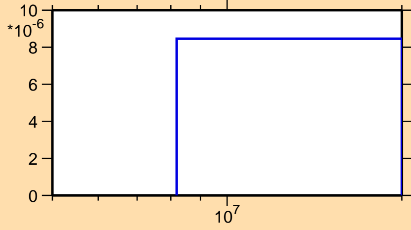
\sigma vs. E for ^{105}\text{Nb}(n,np)
