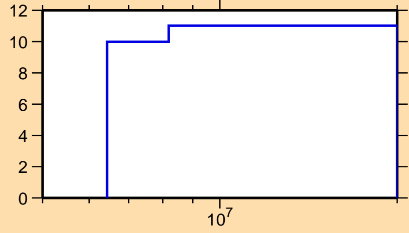
\Delta\sigma/\sigma vs. E for ^{105}\text{Nb}(n,el.)
