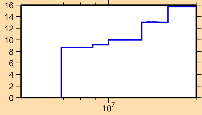
\Delta\sigma/\sigma vs. E for ^{106}\text{Nb}(n,el.)
