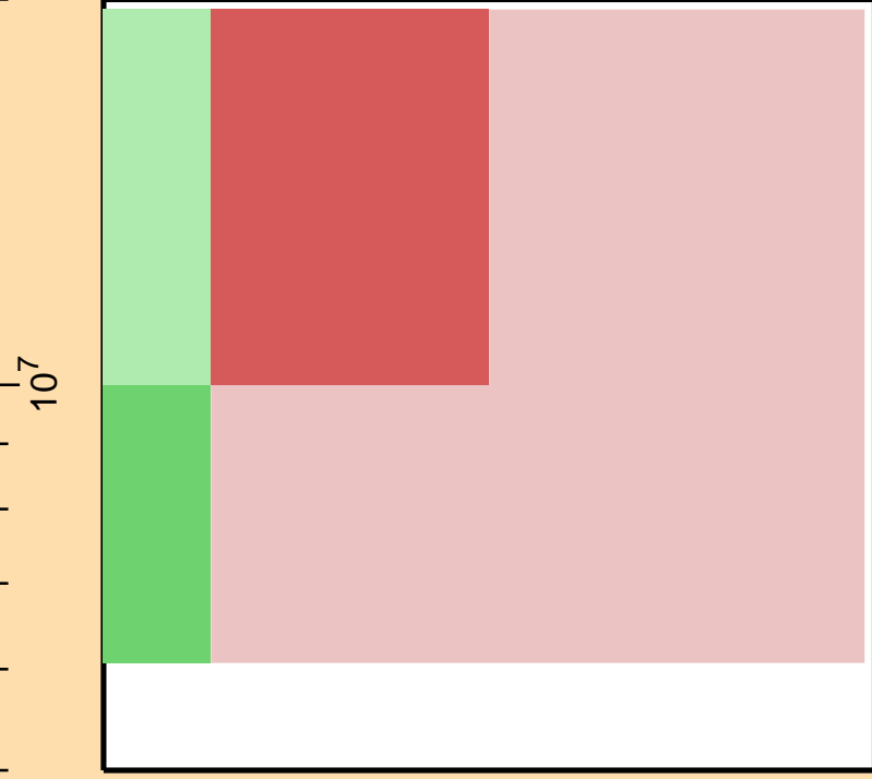
\Delta\sigma/\sigma vs. E for ^{106}\text{Nb}(n,\text{tot.})
