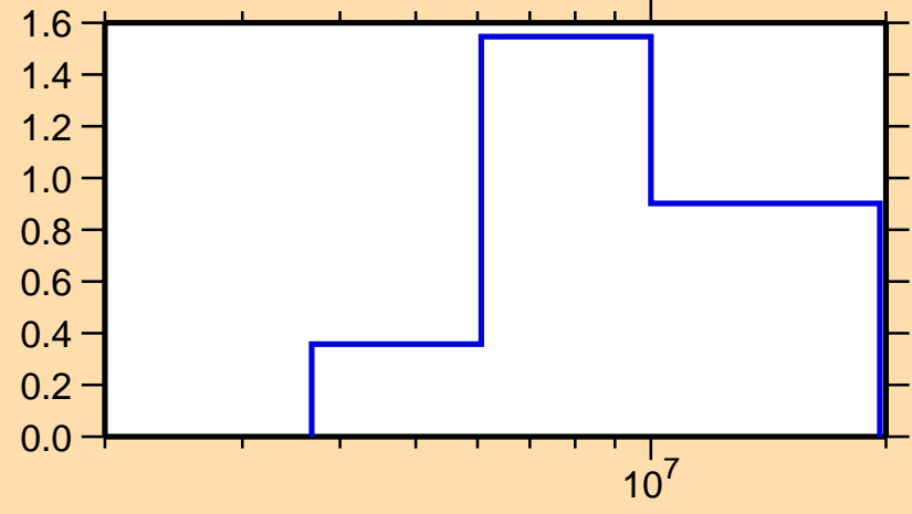
\sigma vs. E for ^{106}\text{Nb}(n,2n)
