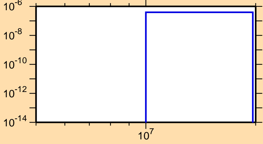
\sigma vs. E for ^{106}\text{Nb}(n,n\alpha)
