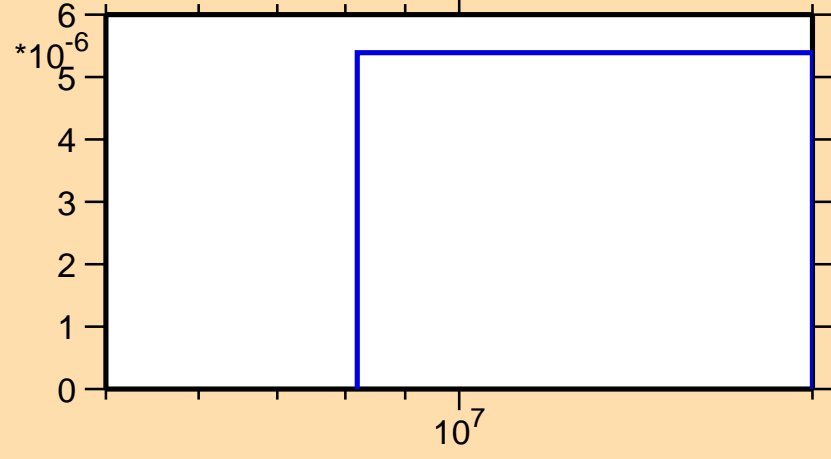
\sigma vs. E for ^{106}\text{Nb}(n,np)
