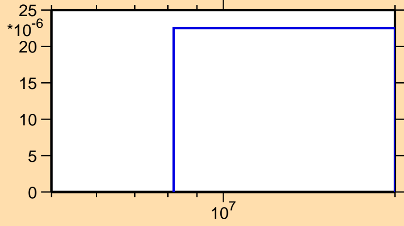
\sigma vs. E for ^{106}\text{Nb}(n,d)
