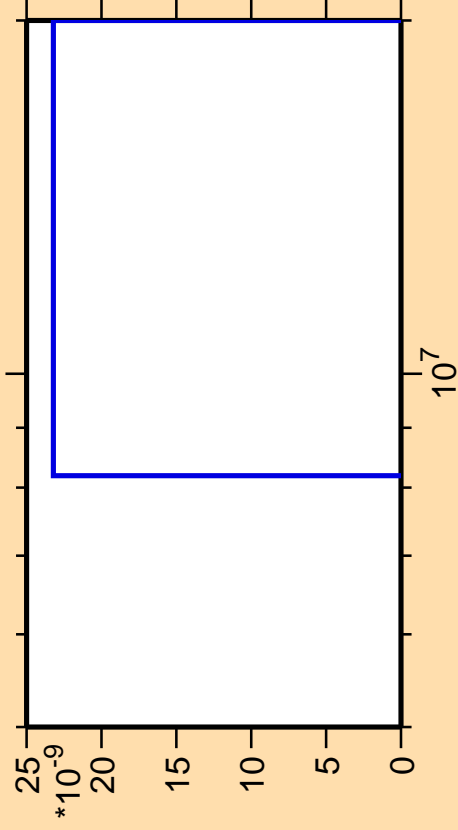
\Delta\sigma/\sigma vs. E for ^{106}\text{Nb}(\text{mt } 11)
