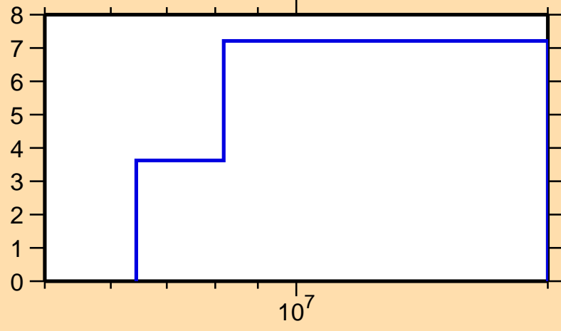
\Delta\sigma/\sigma vs. E for ^{106}\text{Nb}(n,\text{tot.})
