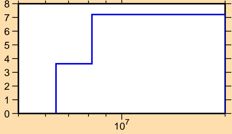
\Delta\sigma/\sigma vs. E for ^{106}\text{Nb}(n,\text{tot.})
