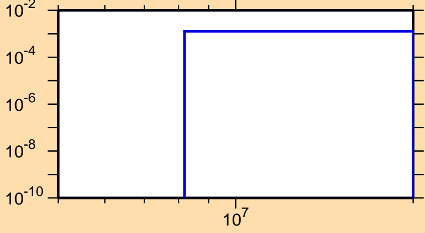
\sigma vs. E for ^{106}\text{Nb}(n,p)
