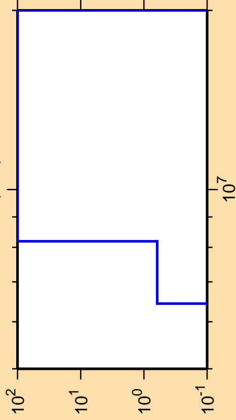
\Delta\sigma/\sigma vs. E for ^{106}\text{Nb}(n,\alpha)
