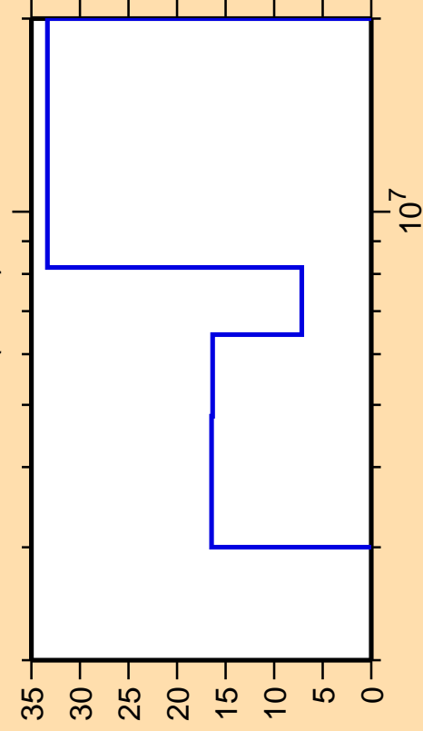
\Delta\sigma/\sigma vs. E for ^{106}\text{Nb}(n,2n)
