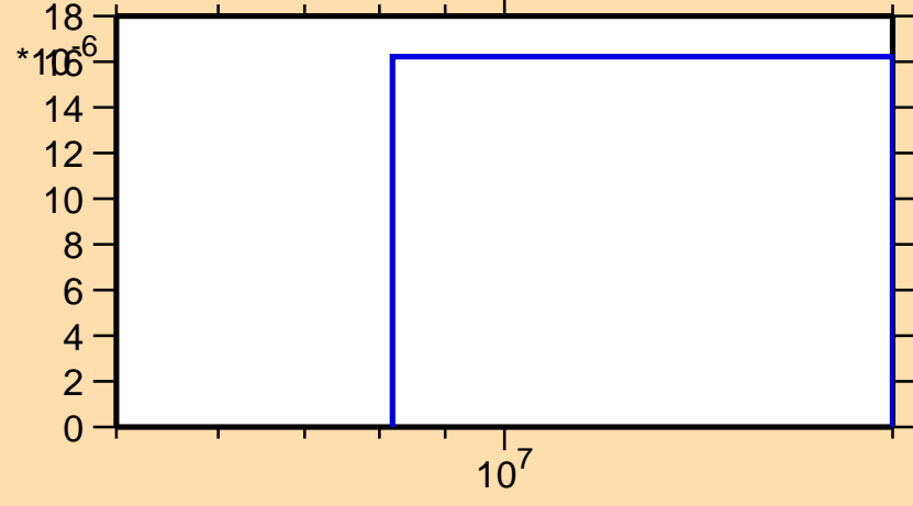
\sigma vs. E for ^{106}\text{Nb}(n,t)
