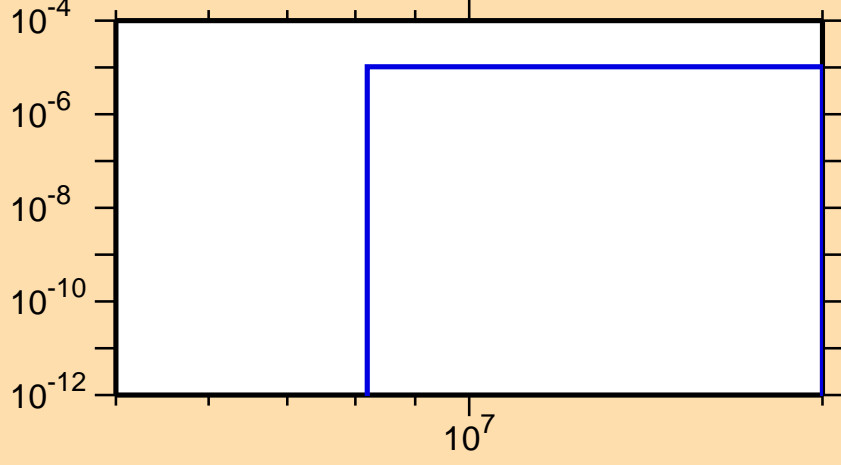
\sigma vs. E for ^{106}\text{Nb}(n,\alpha)
