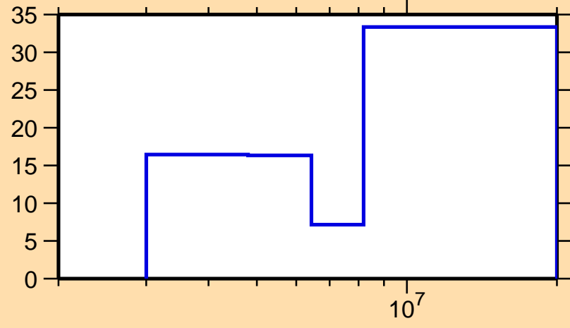
\Delta\sigma/\sigma vs. E for ^{106}\text{Nb}(n,2n)
