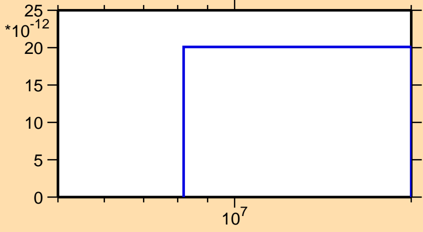
\sigma vs. E for ^{106}\text{Nb}(n,2n\alpha)
