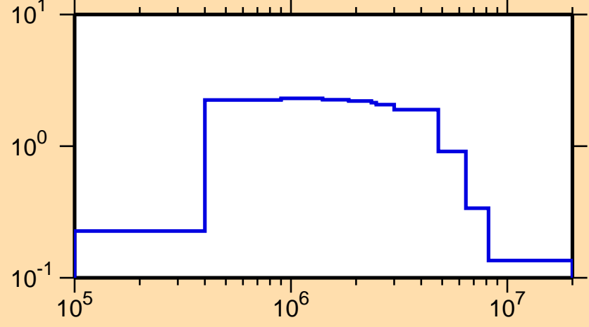
\sigma vs. E for ^{106}\text{Nb}(n,n_{\text{cont}}) .
