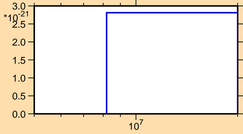
\sigma vs. E for ^{106}\text{Nb}(\text{mt } 11)
