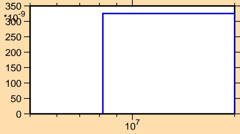
\sigma vs. E for ^{106}\text{Nb}(n,n\alpha)
