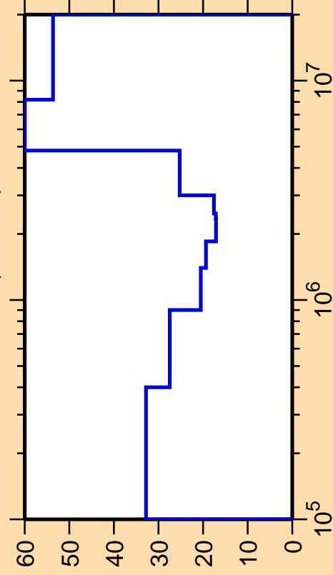
\Delta\sigma/\sigma vs. E for ^{106}\text{Nb}(n,\text{inel.})
