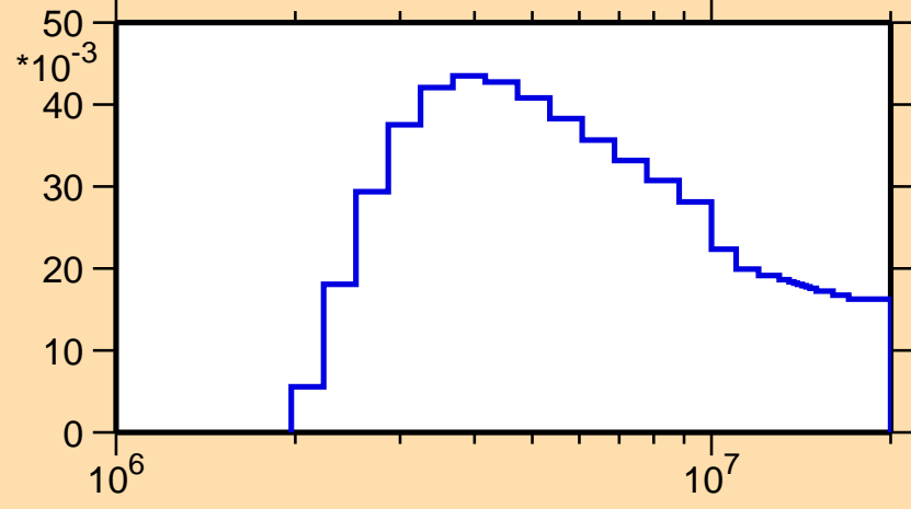
\sigma vs. E for ^{18}\text{Ne}(n,n_1)
