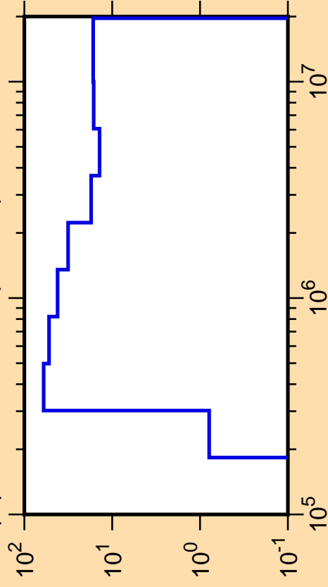
\Delta\mu/\mu vs. E for ^{18}\text{Ne}(\text{mt251})
