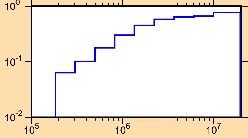
\mu vs. E for ^{18}\text{Ne}(\text{mt251})
