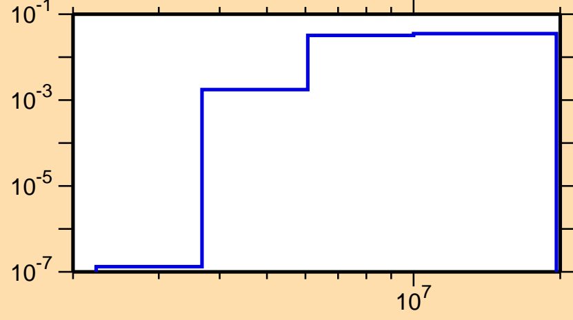
\sigma vs. E for ^{18}\text{Ne}(n,\text{pd})
