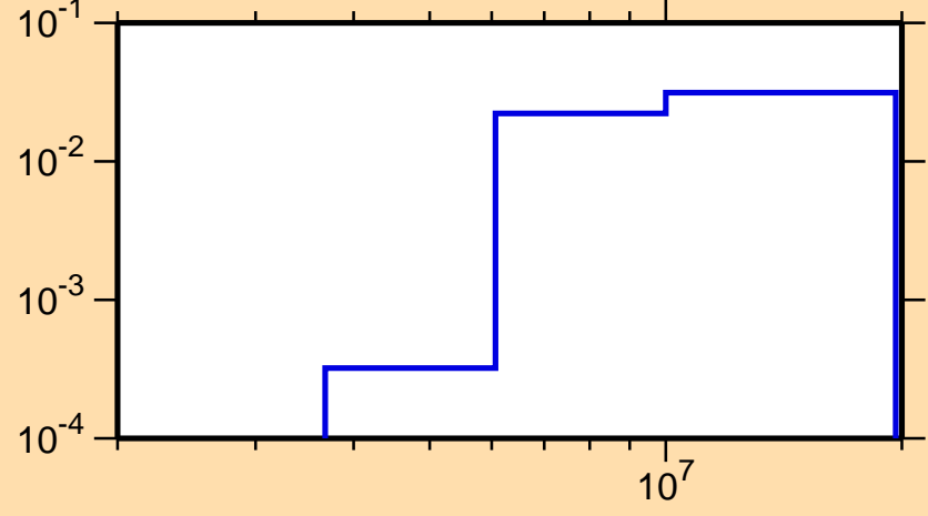
\sigma vs. E for ^{18}\text{Ne}(n,np)
