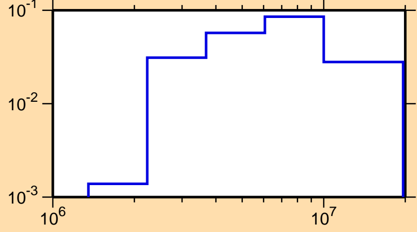
\sigma vs. E for ^{18}\text{Ne}(n,\text{inel.})
