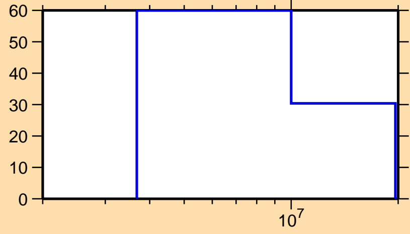
\Delta\sigma/\sigma vs. E for ^{18}\text{Ne}(n,ncont.)
