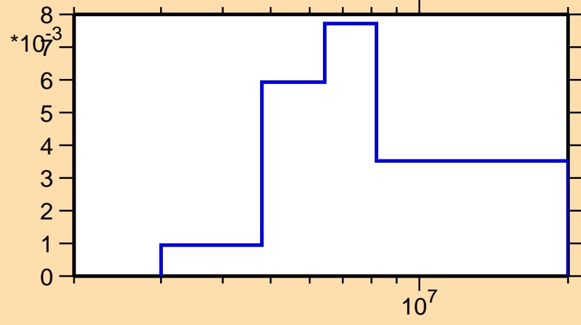
\sigma vs. E for ^{18}\text{Ne}(n,n_2)
