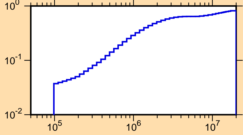
\mu vs. E for ^{19}\text{Ne}(\text{mt251})
