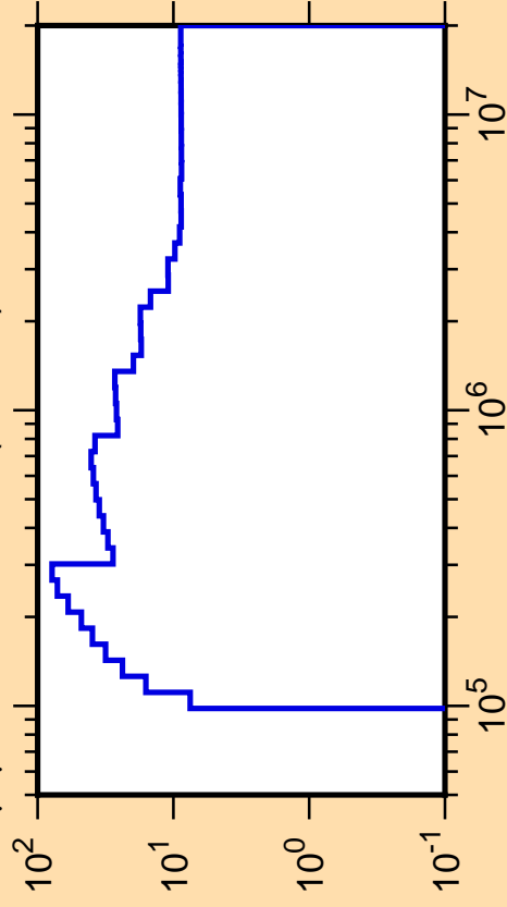
\Delta\mu/\mu vs. E for ^{19}\text{Ne}(\text{mt251})
