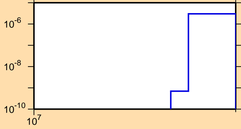
\sigma vs. E for ^{19}\text{Ne}(n,2np)
