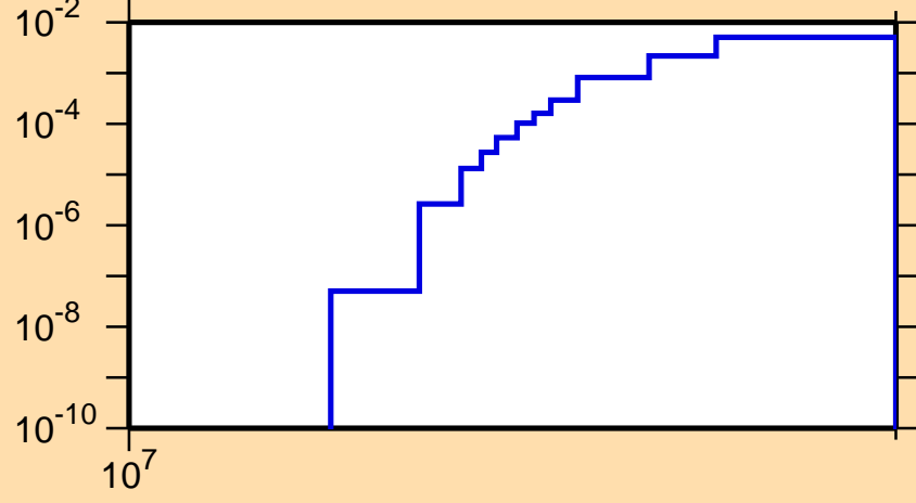
\sigma vs. E for ^{19}\text{Ne} (mt 45)
