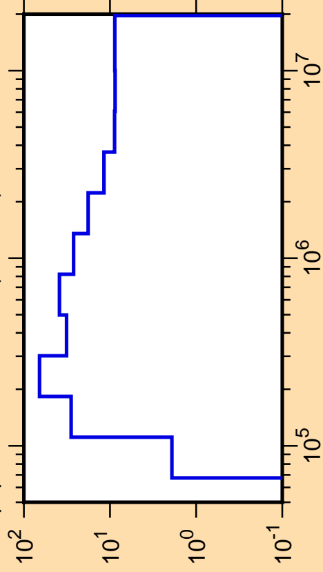
\Delta\mu/\mu vs. E for ^{19}\text{Ne}(\text{mt251})
