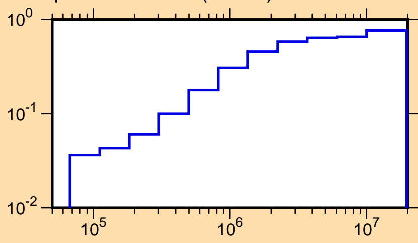
\mu vs. E for ^{19}\text{Ne}(\text{mt251})
