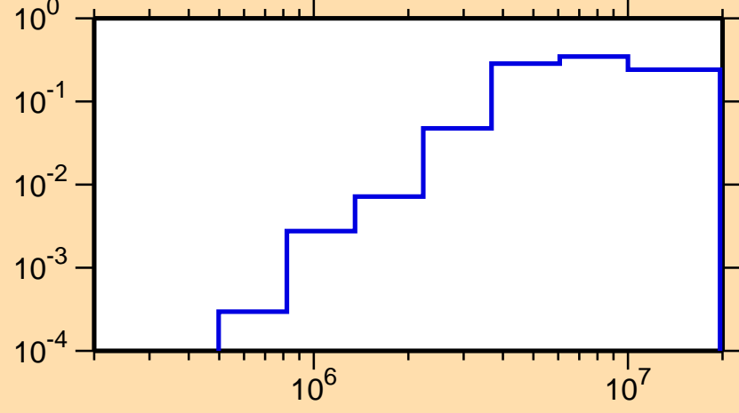
\sigma vs. E for ^{20}\text{Ne}(n,\alpha)
