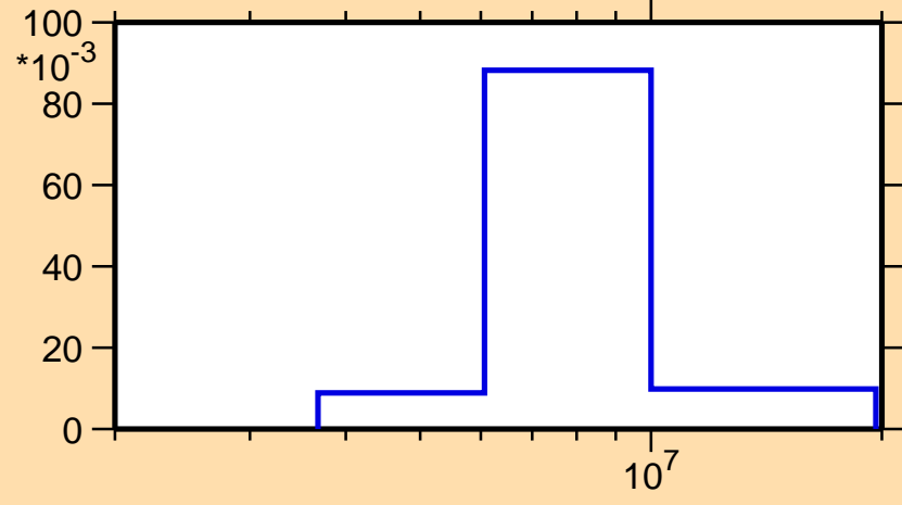
\sigma vs. E for ^{20}\text{Ne}(n,n_3)
