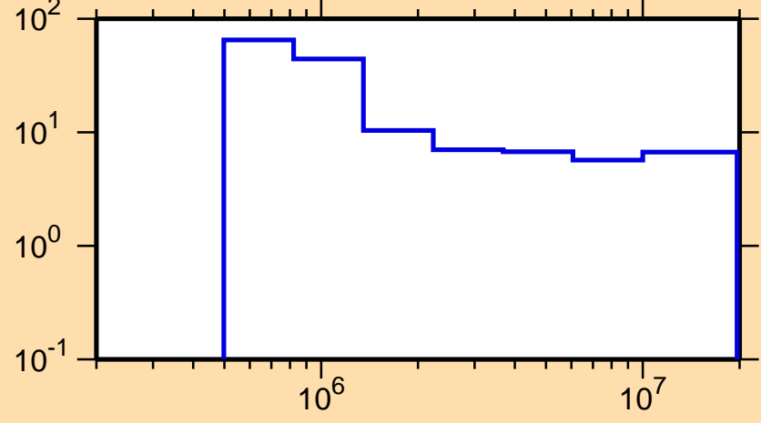
\Delta\sigma/\sigma vs. E for ^{20}\text{Ne}(n,\text{nonel.})
