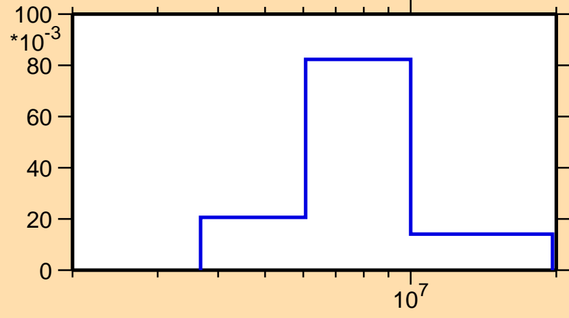
\sigma vs. E for ^{20}\text{Ne}(n,n_2)
