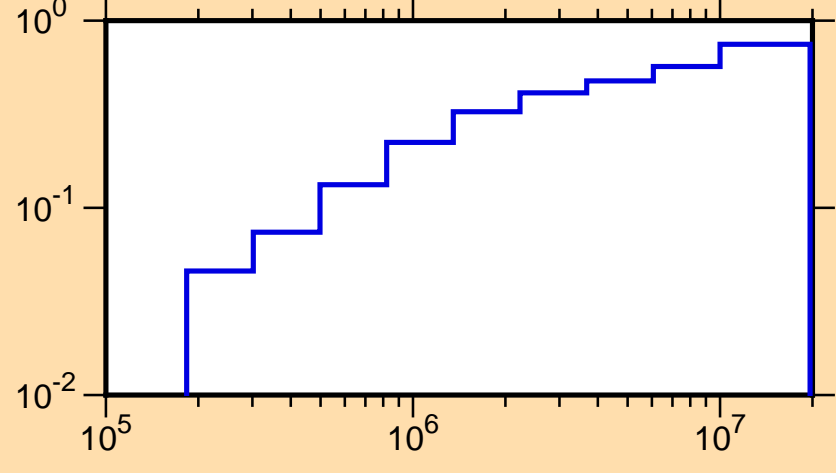
\mu vs. E for ^{21}\text{Ne}(\text{mt251})
