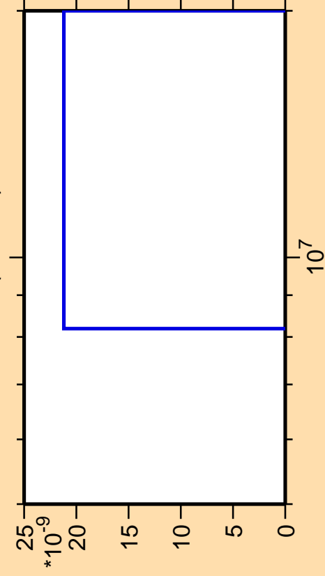
\Delta\sigma/\sigma vs. E for ^{21}\text{Ne}(\text{mt117})
